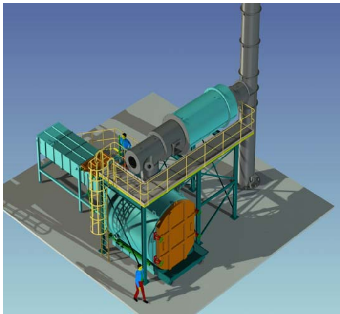
Model RD1000 Dual-fired Incinerator - throughput 1000 kg per hour
