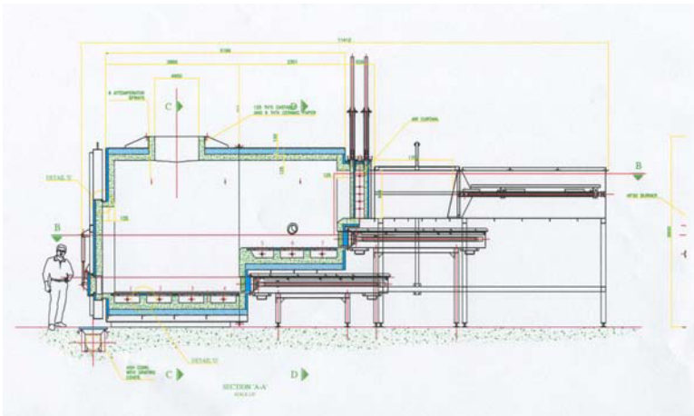
Special engineered RD1000 pyrolytic incinerator
